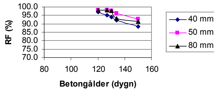
Betong-RF Rum 1:28
