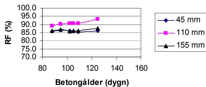
Betong-RF Rum 2:7
